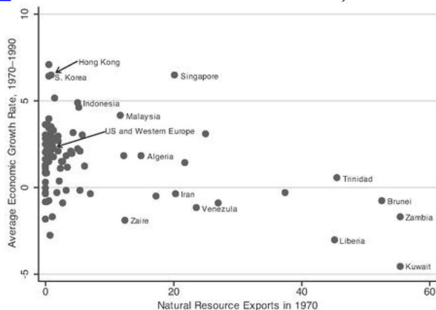
FIGURE 4.2 Growth and Natural Resource Abundance, 1970–1990
